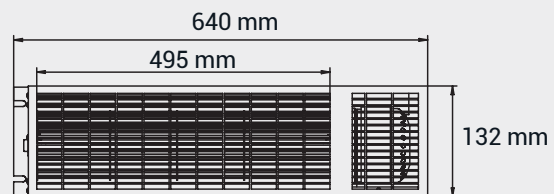
FAN3300S
